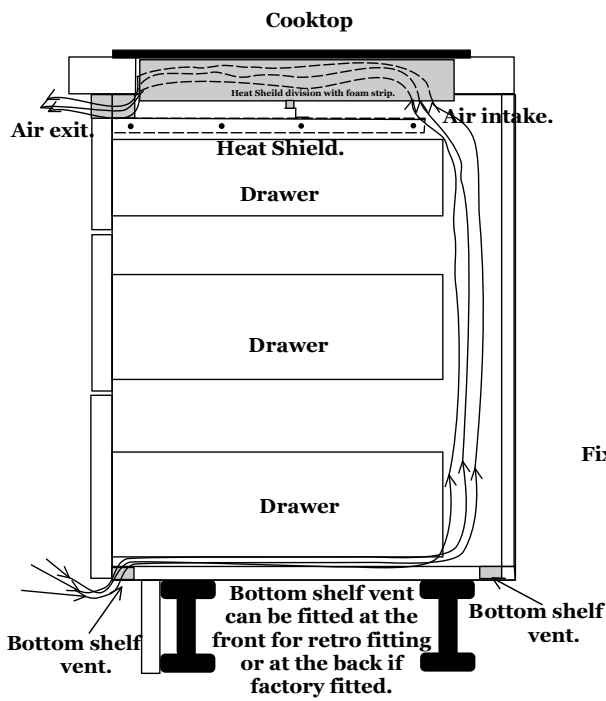
Bottom shelf vent in mesh.
